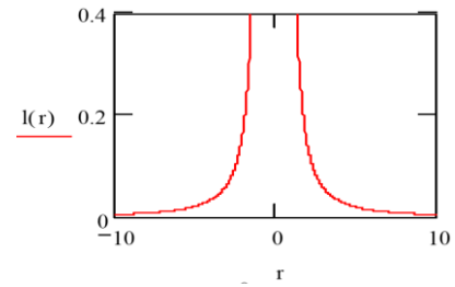
Fig. 3: Graph of the function of relative elongation of the outer side of the \lambda_{12,15} -vacuum (i.e. subcont) in the outer shell of a moving "electron" in the radial direction (37) l_r^{(+)} = \Delta r/r at r_6 = 1 and V_z/c = 0.007 , V_z/c = 0.0007 , V_z/c = 0.00007
