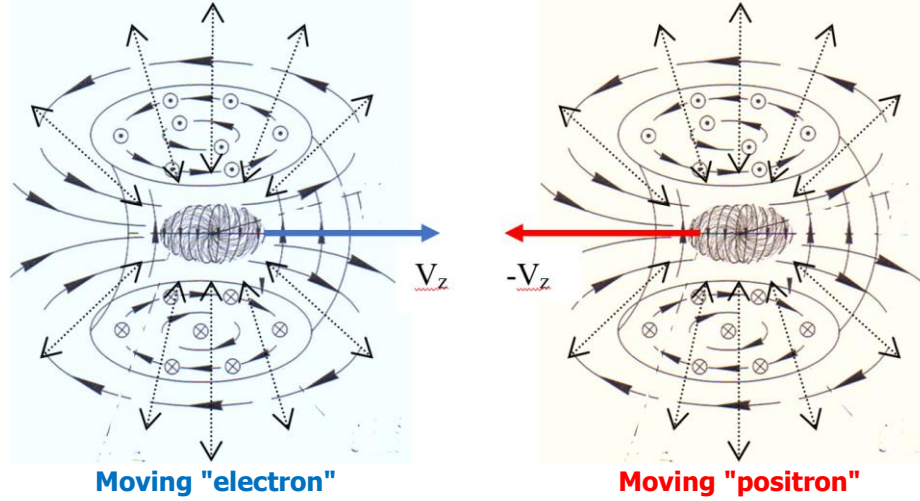
Fig. 16: "Electron" and "positron" moving rectilinearly and uniformly with the same speed V_z , but in opposite directions. In this case, all processes (i.e. accelerated laminar and turbulent flows) in their outer shells completely coincide
