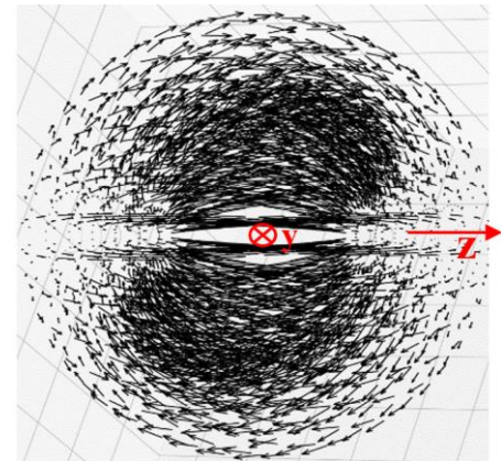
Fig. 5.2: The cross-section of the field of the velocity component v_\phi^{(+b1)} of the b_1 -subcontact is rotated by 90^\circ around the Z axis
