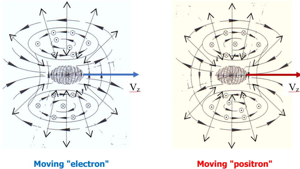
Fig. 15: "Electron" and "positron" moving rectilinearly and uniformly with the same speed V_z in the same direction. In this case, all processes (i.e. accelerated laminar and turbulent flows) in their outer shells are mutually opposite
