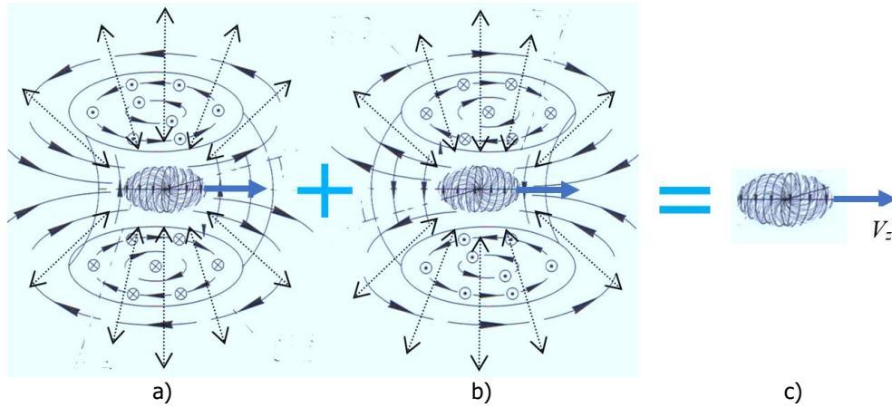
Fig. 7: In the outer shell (more precisely in the vicinity of the core) of an "electron" moving at a constant speed V_z on average, two counter toroidal-helical subcont vortices and two counter (inflowing and outflowing) subcont laminar currents are induced, which compensate for each other's manifestations
