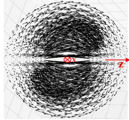
Fig. 5.1: The cross-section of the field of the velocity component v_{\phi}^{(+a1)} of the a_1 -subcont. Calculations were performed using the Mathplotlib library
