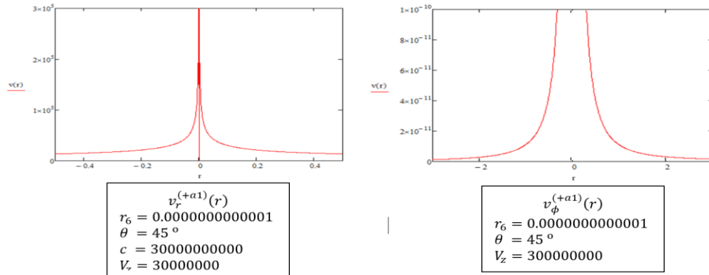
Fig. 6.1: Graphs of functions v_r^{(+a1)}(r) and v_{\phi}^{(+a1)}(r) (45)
