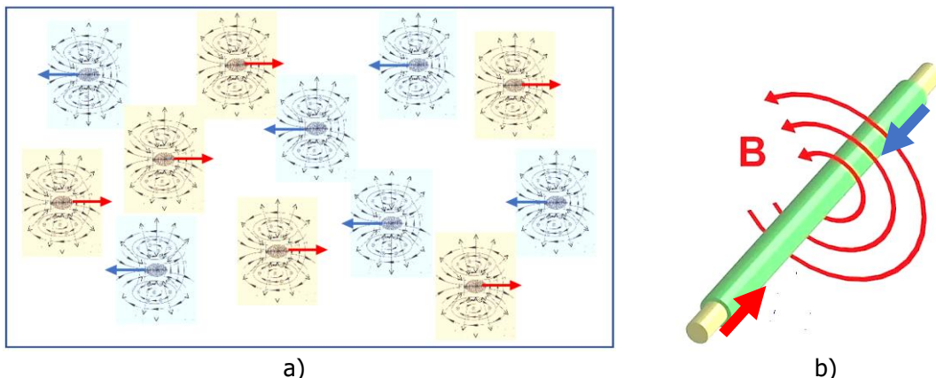
Fig. 20: "Particles" and "antiparticles" (in particular, "electrons" and "positrons") moving in a metal wire rectilinearly and uniformly with the same speed V/2 towards each other, i.e. in opposite directions. At the same time, their counter toroidal-helical vortices rotate in one direction
