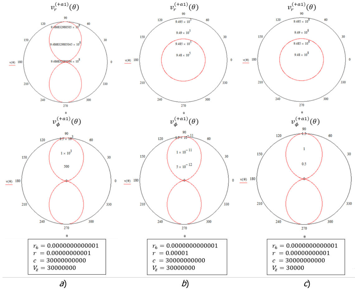
Fig. 6.2: Graphs of functions v_r^{(+a1)}(\theta) and v_\phi^{(+a1)}(\theta) (45) for different values of parameters r, V_z
