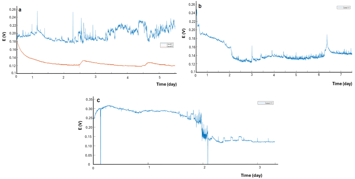
Fig. 4: Voltage (V) versus Time (dias) Measurement. (a) Electrodes 5 \times 1 \text{ cm}^2 , spaced 5 cm (blue) and 2 cm (red). (b) Electrodes 5 \times 0.5 \text{ cm}^2 , spaced 2 cm. (c) Electrodes 5 \times 0.5 \text{ cm}^2 , spaced 5 cm.
