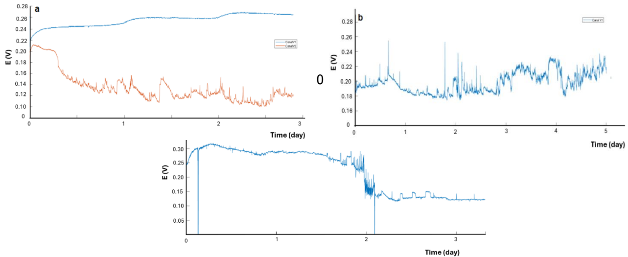
Fig. 3: Potential Measurement (V) versus Time (dias). (a) Electrodes 15 \times 5 \text{ cm}^2 (blue line) and 10 \times 5 \text{ cm}^2 (orange line), (b) Electrodes 5 \times 1 \text{ cm}^2 . (c) Electrodes 5 \times 0.5 \text{ cm}^2 .
